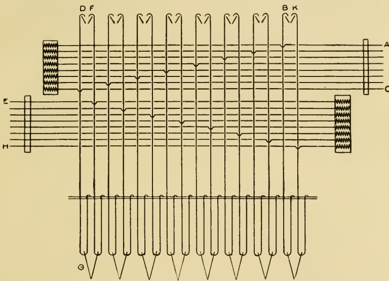
Fig. 27. Arrangement of Needles and Hooks in Double Action Machine.
